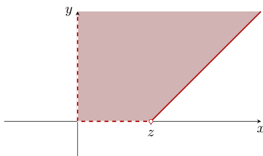
Figure 14.3: Let z > 0 . The region in \mathbb{R}^2 corresponding to the event \{X - Y \leq z\} for positive random variables X and Y .
